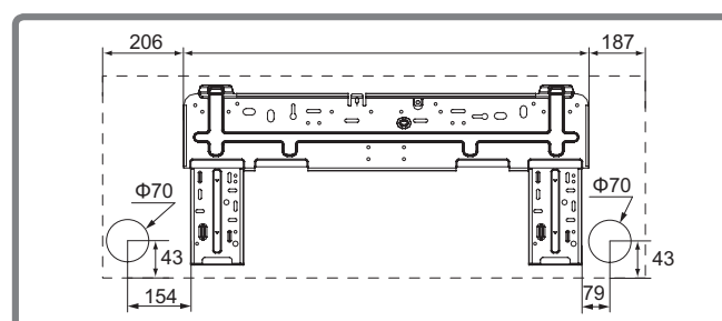
7,0 kW
